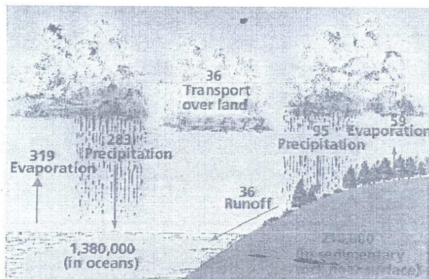
Fig. 4.1 The Hydrological Cycle
